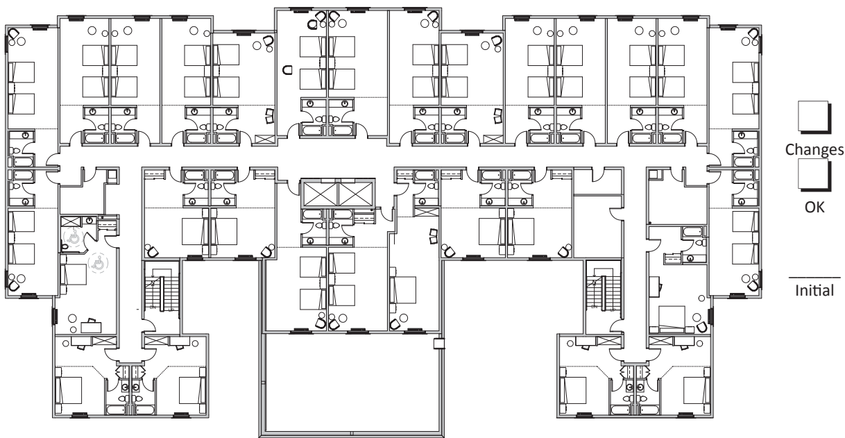
Third Floor
